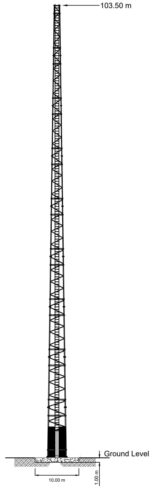
10.00 m 2 Raft Foundation
